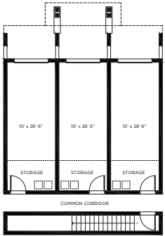
GARAGE PLAN
